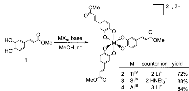
Scheme 1. Synthesis of octupolar (catecholato) M IV,III complexes 2–4 .
