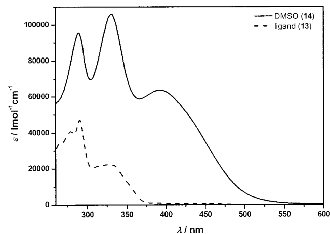
Figure 4. Absorption spectra of tris(catecholato)M complex 14 and ligand 13 in DMSO.
