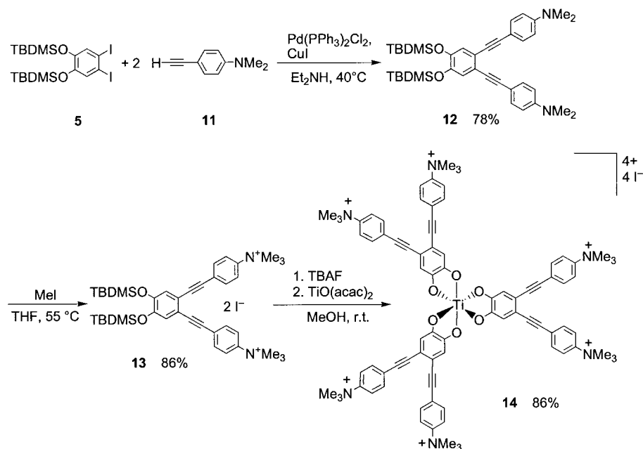
Scheme 3. Syntheses of the TBDMS-protected acceptor-substituted catechol ligand 13 and the corresponding octupolar Ti IV complex 14 .
