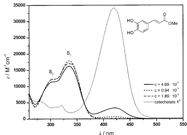
Figure 1. Concentration-dependent UV/Vis spectra of 1 and the catecholate 12 − in DMSO.
