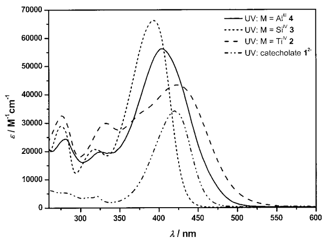
Figure 2. Absorption spectra of tris(catecholato)M complexes 2–4 and of catecholate 12 - in DMSO.
