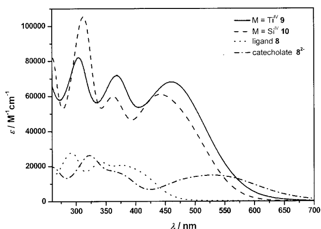
Figure 3. Absorption spectra of the tris(catecholato)M complexes 9 , 10 and the corresponding ligand 8 and catecholate 8 2- in DMSO.
