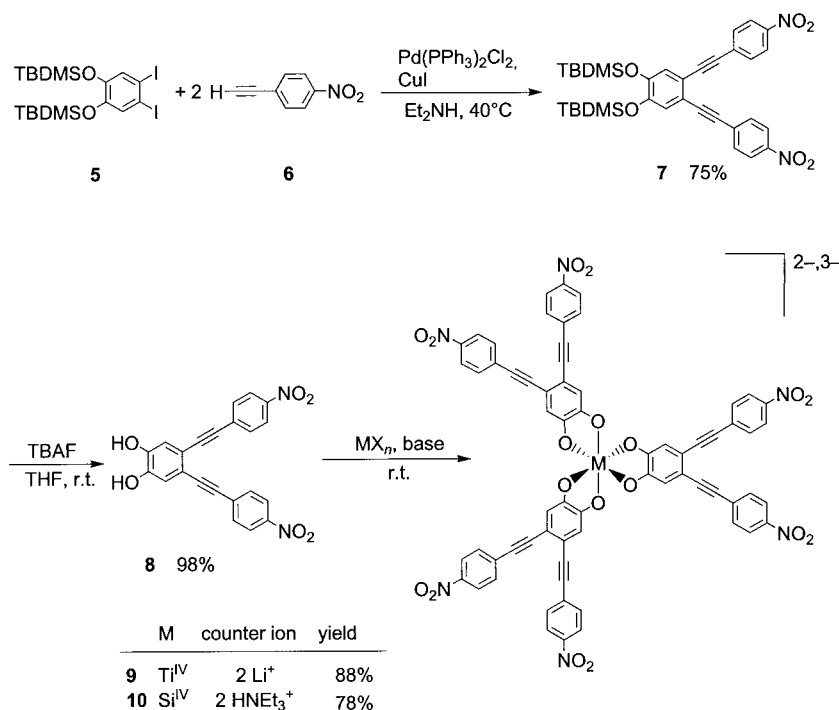
Scheme 2. Syntheses of the acceptor-substituted catechol ligand 8 and the corresponding octupolar Ti IV ( 9 ) and Si IV complexes ( 10 ).
